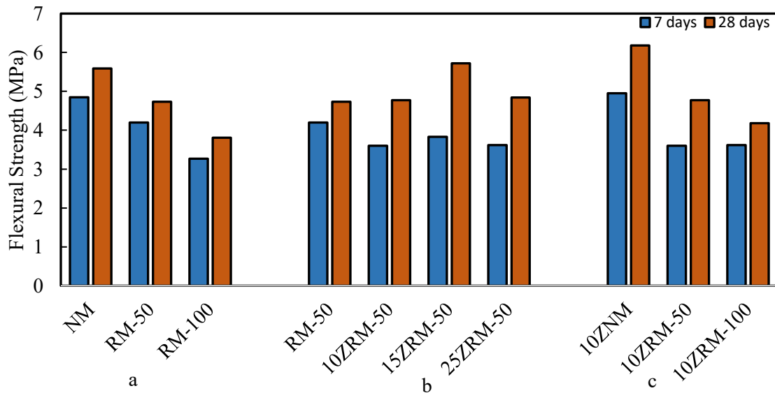
Fig. 5. Flexural strength of 7 and 28-day mortar specimens with increasing substitution of (a) recycled sand in the base scheme, (b) zeolite in the scheme containing equal amounts of natural and recycled sand, and (c) recycled sand in the scheme containing zeolite
