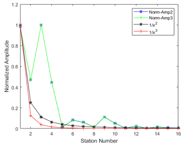
Fig. 3. Effect of geometrical spreading on the amplitudes of first-arrival traveltimes in the seismic refraction data from the forward shot.
