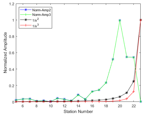
Fig. 4. Effect of geometrical spreading on the amplitudes of first-arrival traveltimes in the seismic refraction data from the reverse shot.
