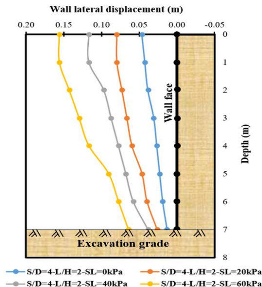
Fig. 11. Effect of surcharge load on the variation of wall lateral displacement versus depth
