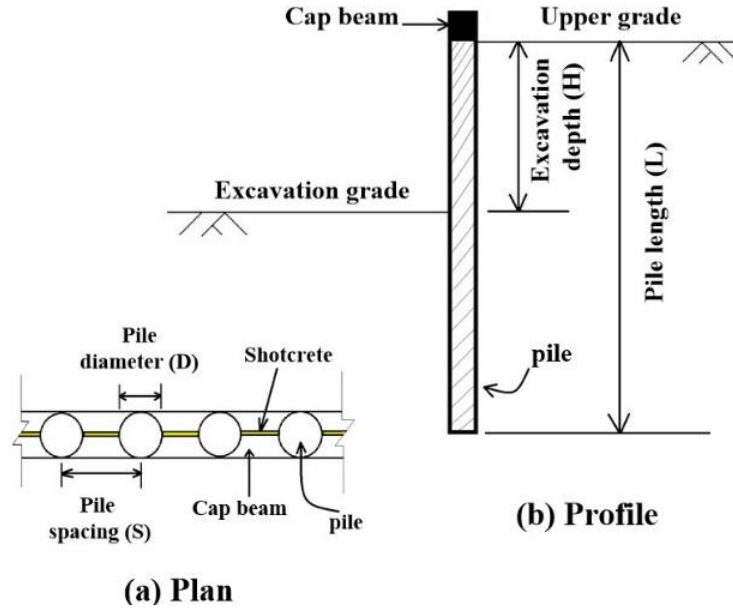
Fig. 1. Cantilever Pile Wall (CPW)
