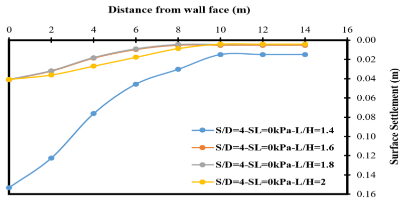
Fig. 9. Effect of pile embedded length on the variation of surface settlement versus distance from the wall face
