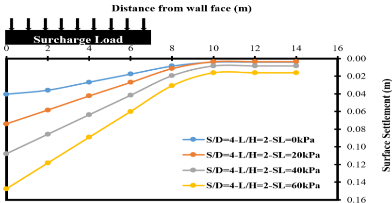
Fig. 12. Effect of surcharge load on the variation of surface settlement versus distance from the wall face
