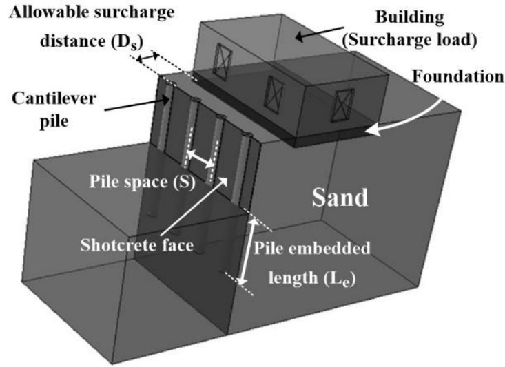
Fig. 2. Excavation and building supported by CPW
