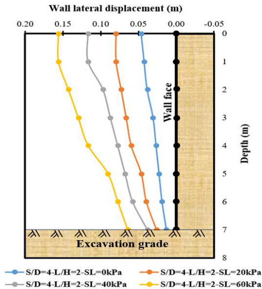
Fig. 11. Effect surcharge load on the variation of wall lateral displacement versus depth
