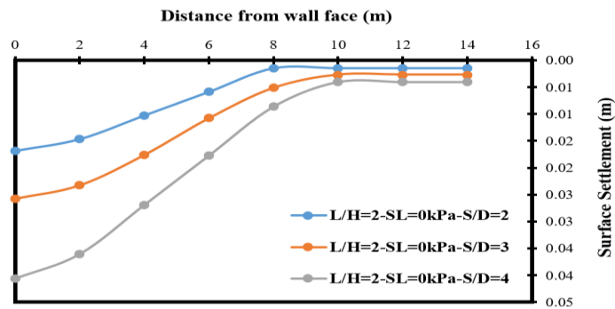
Fig. 6. Effect of pile spacing on the variation of surface settlement versus distance from the wall face
