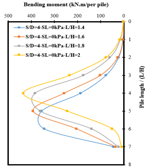
Fig. 7. Effect of pile embedded length on the variation of bending moment along the pile length
