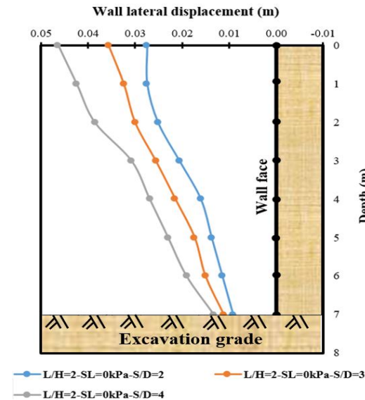
Fig. 5. Effect of pile spacing on the variation of wall lateral displacement versus depth
