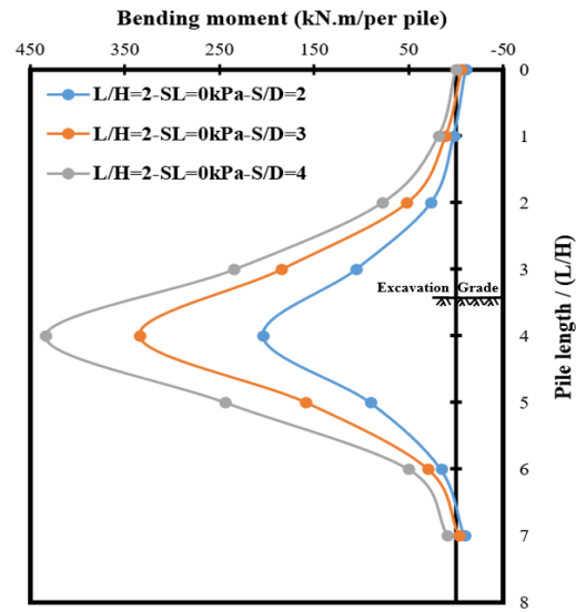
Fig. 4. Effect of pile spacing on the variation of bending moment along the pile length
