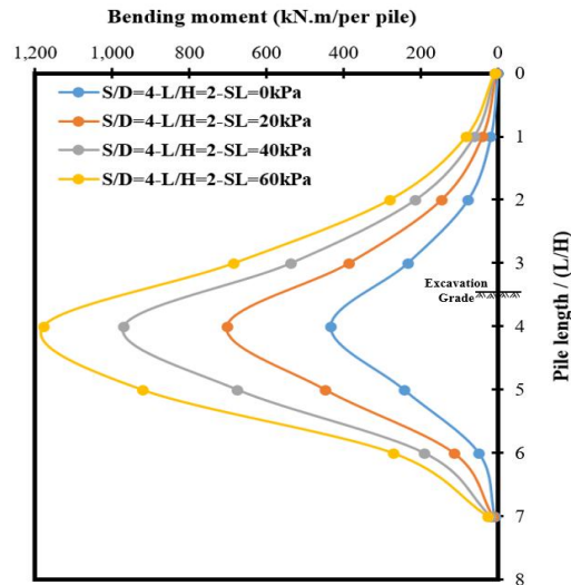
Fig. 10. Effect of surcharge load on the variation of bending moment along the pile length
