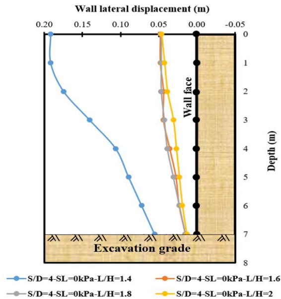
Fig. 8. Effect of pile embedded length on the variation of wall lateral displacement versus depth
