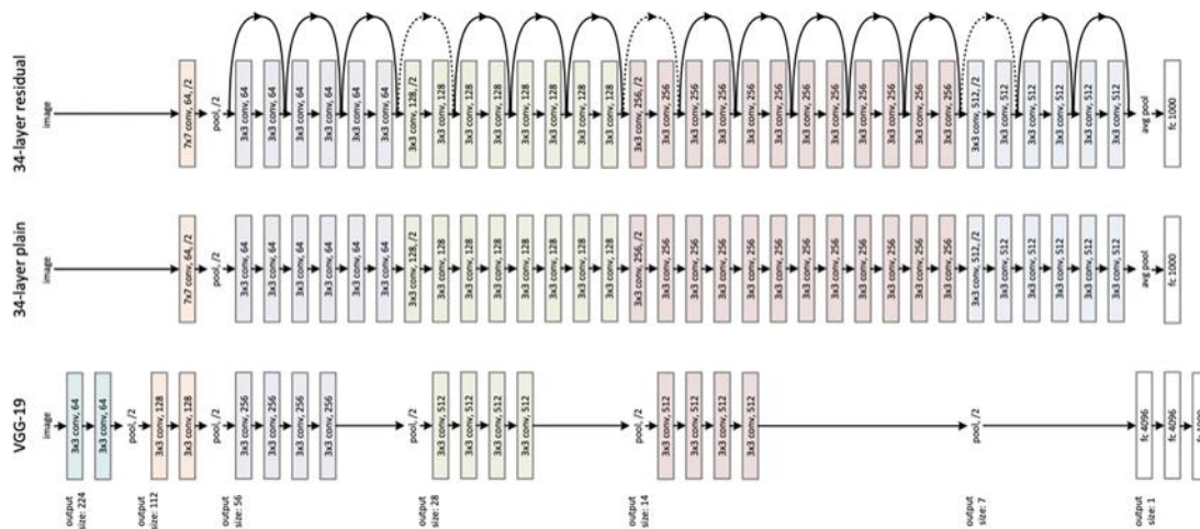
Figure 2. General structure of a ResNet [3]
